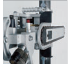
Cutting flush with the wall and non-overlapping corners
