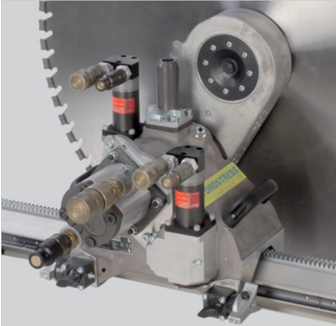
Robust saw head with standard hydraulic motors
