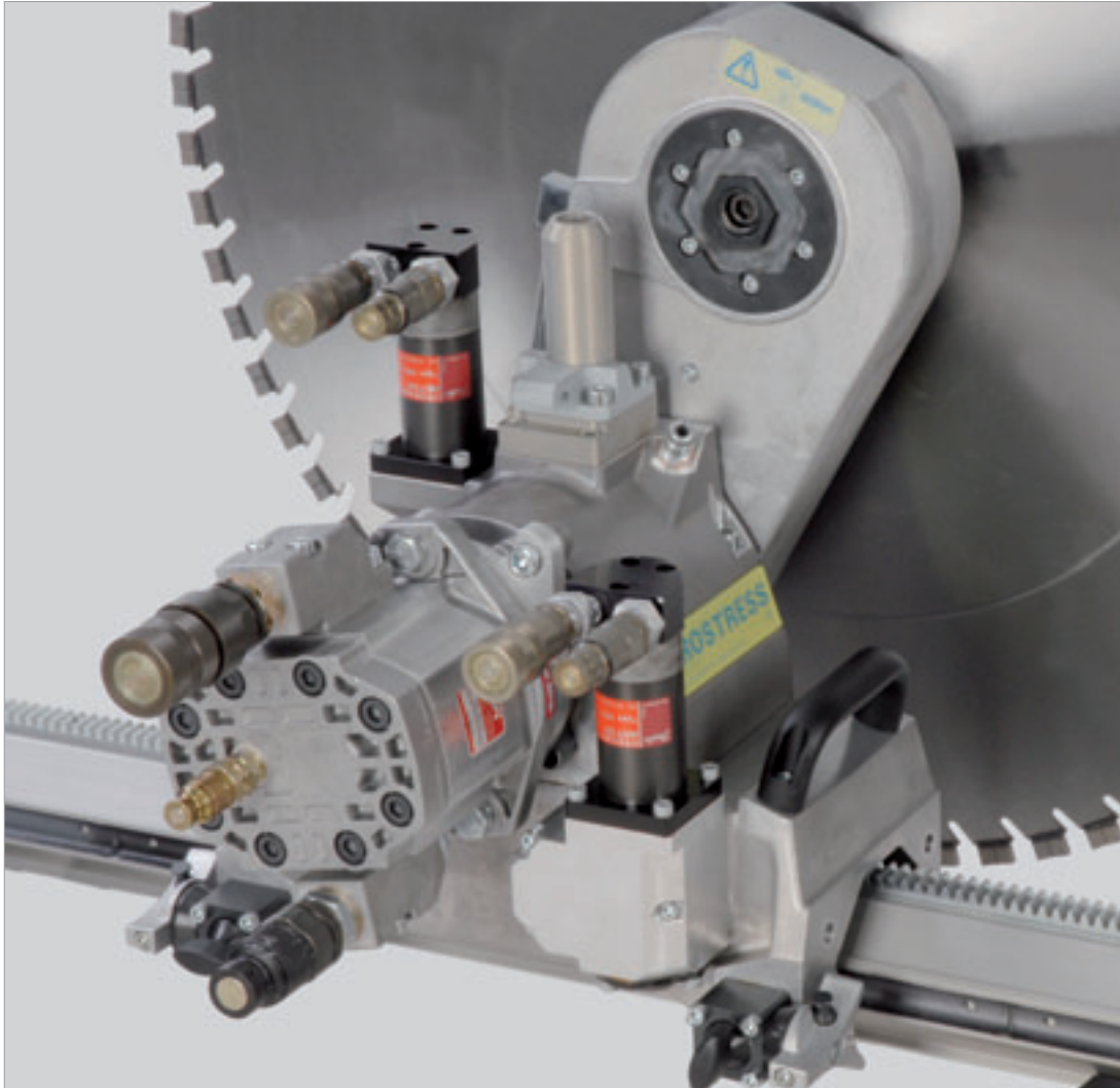
Compact saw head with belt-drive swivel arm
