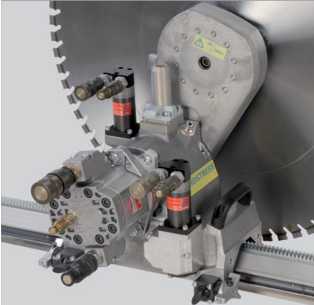
Main motor with leakage oil connection
