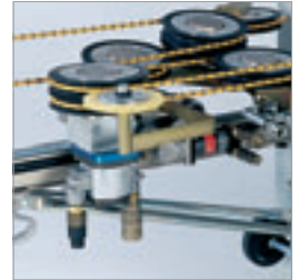
Sophisticated wire store with clamping roll
